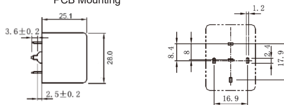
PCB Mounting
