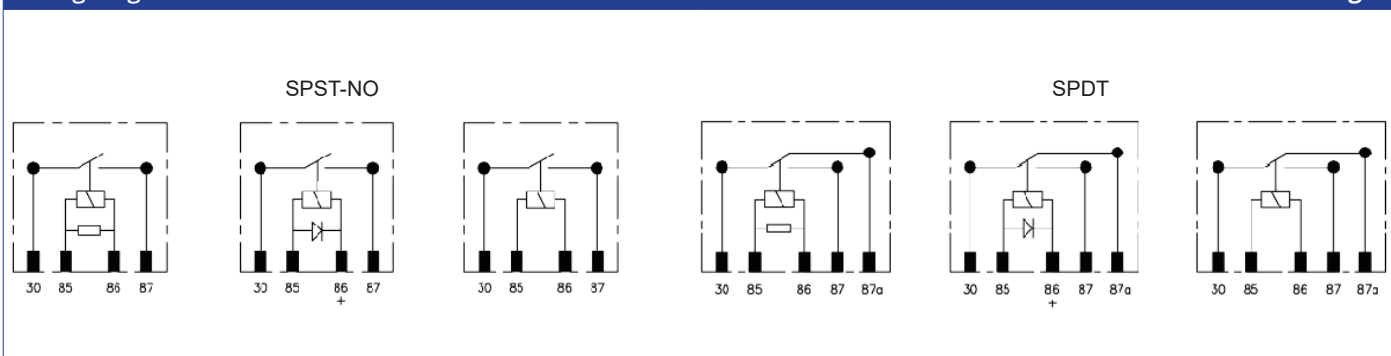
Wiring diagram
