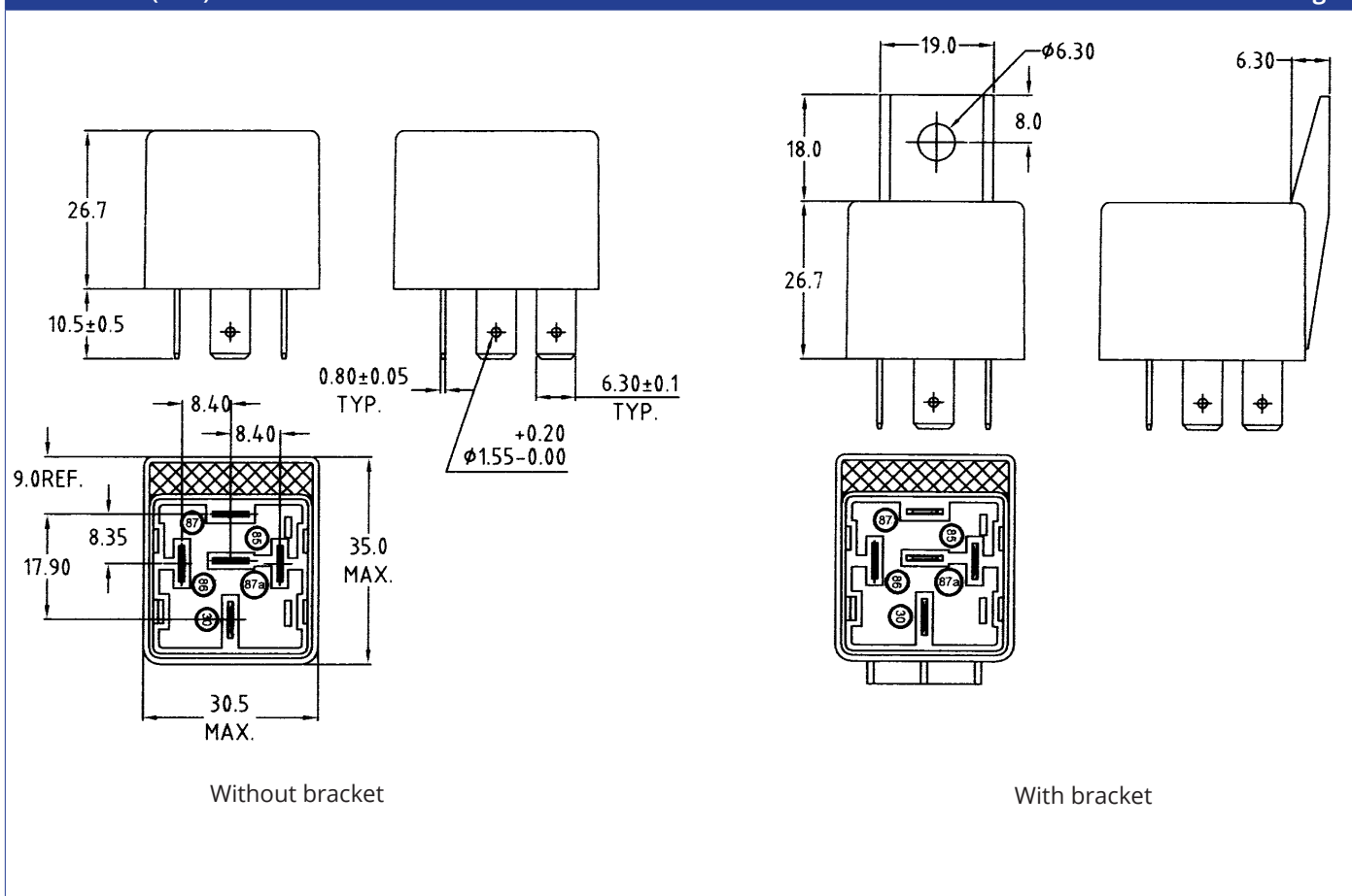
Dimensions (mm)
