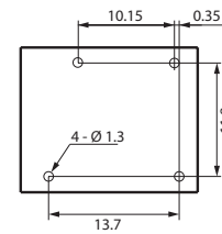
PCB Mounting Dimensions mm (bottom view)
