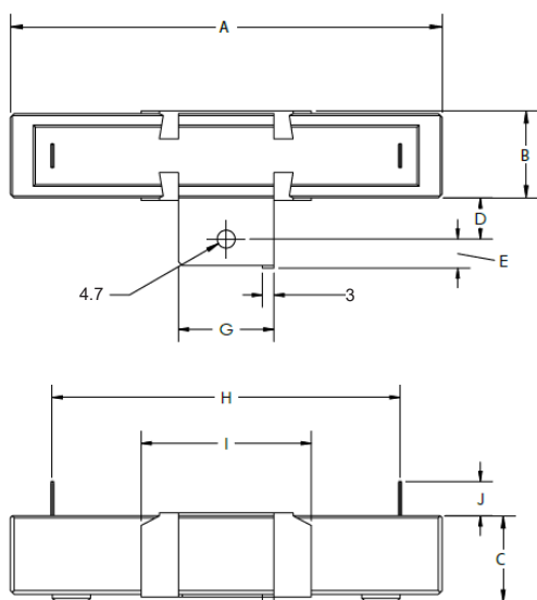
Dimensions (mm) ± 1mm
