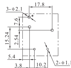
PCB Mounting Dimensions mm
