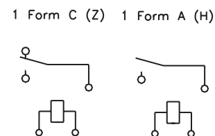
Wiring Diagrams (bottom view)
