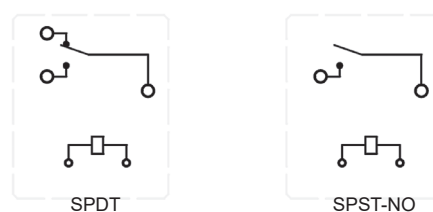
Wiring Diagrams (bottom view)
