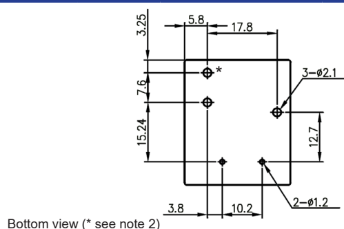
PCB Mounting Dimensions mm
