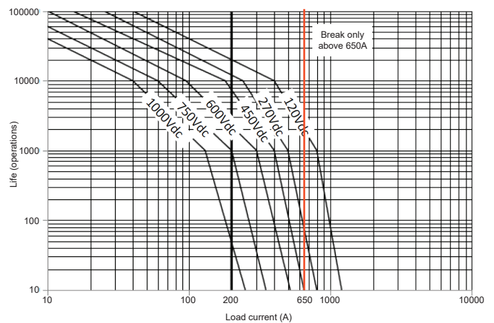
Electrical Life: Resistive load, non-polarized types only
