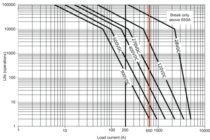
Electrical life: Resistive load, polarized types only
